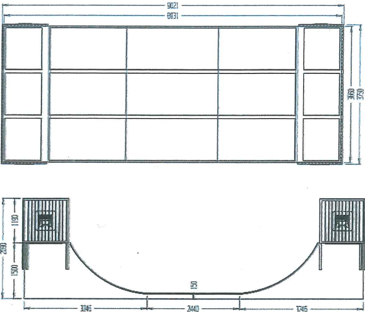
2. KOMPAN CLIMBER - GXY901012
